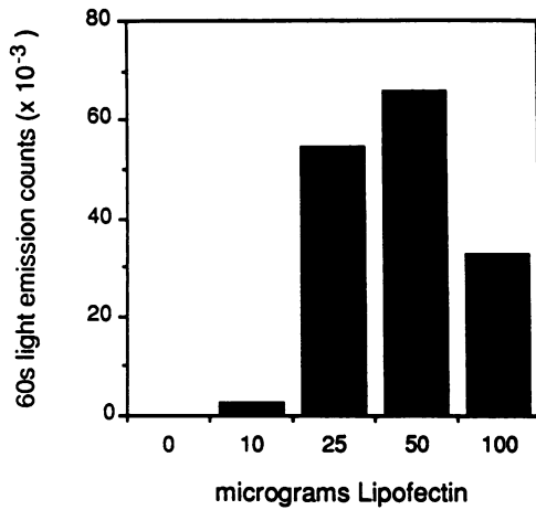
FIG. 2. Transfection efficiency varies with the ratio of RNA to lipofectin. Subconfluent 10-cm plates of NIH 3T3 cells were transfected with 20 µg of RNA (5 µg of Cap-βg Luc βg An + 15 µg of carrier) complexed with various quantities of lipofectin liposomes. Thirty micrograms of total cellular lysate protein from each transfection was then analyzed for luciferase light emission with integration over a 30-s counting interval. Data shown represent the average specific activity of two transfections after correction for background.
